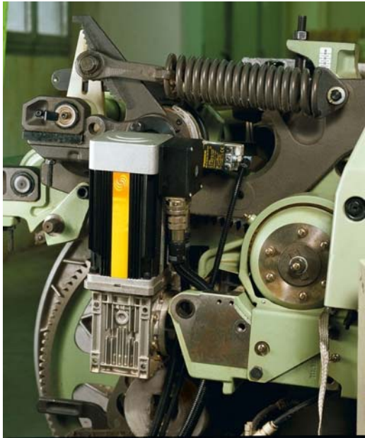
WARP LET-OFF
